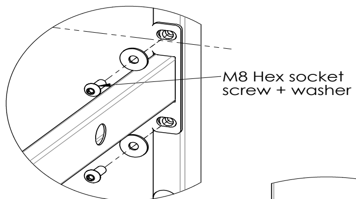
DETAIL A SCALE 1 : 3
