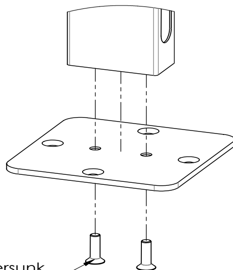
DETAIL C SCALE 1 : 3
