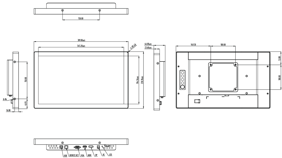
ProLite TF1634MC-B8X without brackets
