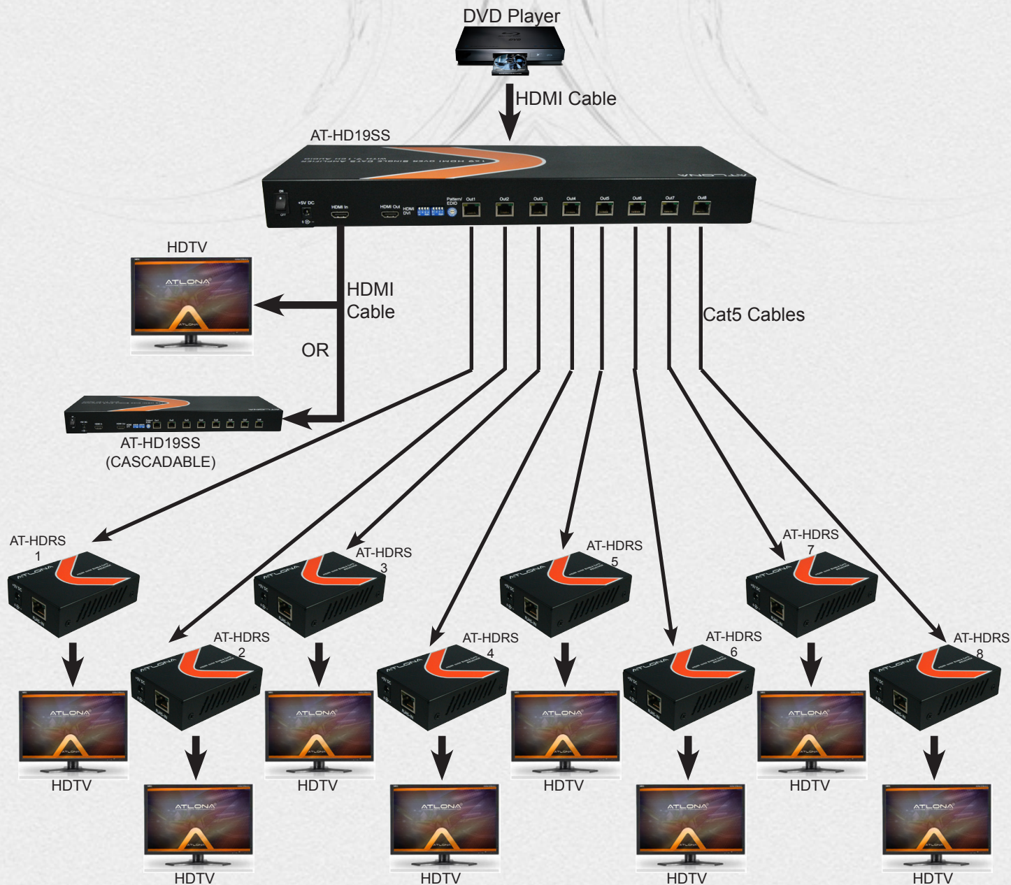
Connection Diagram
