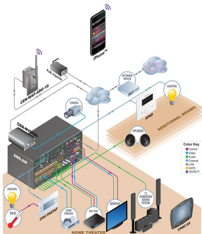
Crestron Mobile Pro® Typical Integration
