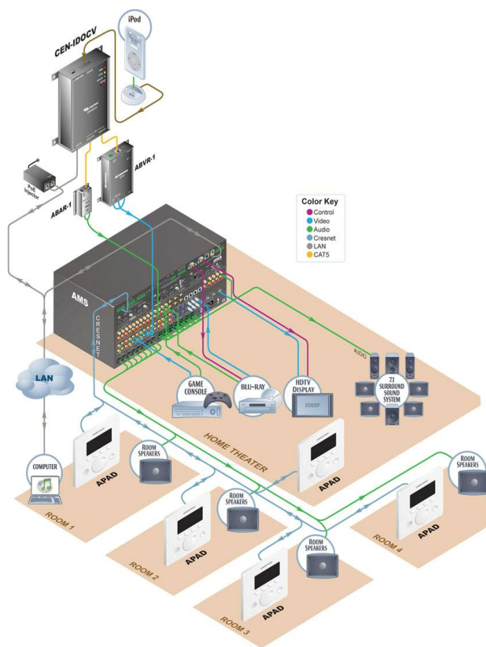
CEN-IDOCV with AMS
