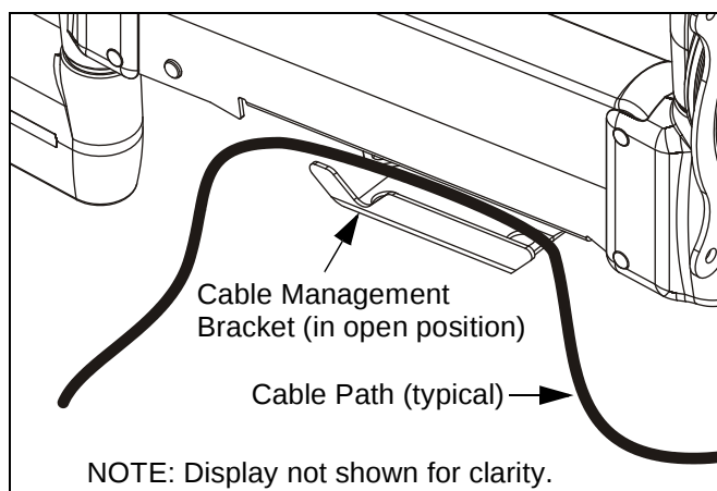
Figure 21: Height Adjustable Arm - Cable Path
