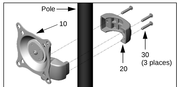
Figure 9: Pole Mount Installation
